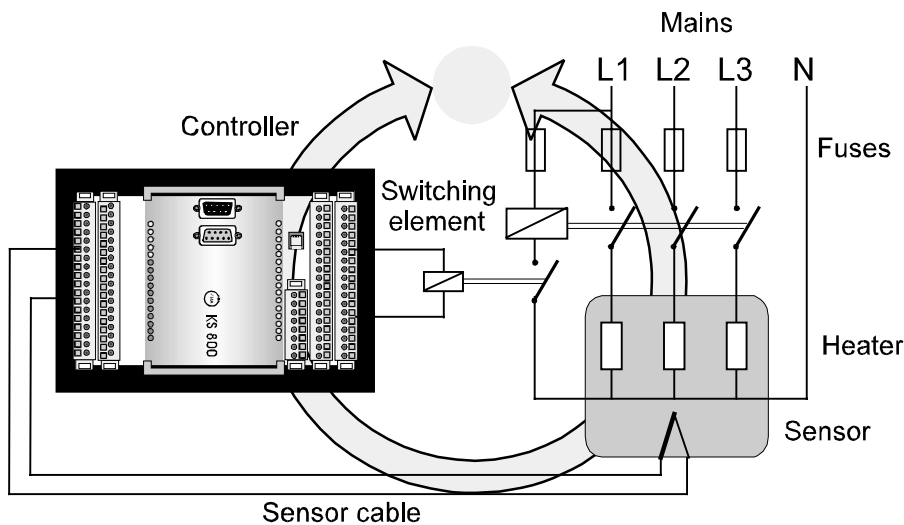
Closed loop monitoring (Loop-Alarm)
