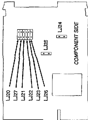
Figure 6-6 Options Board 468 - Link Jumpers
